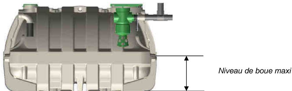
Figure 36ter : Fosse septique PURFLO POWER
